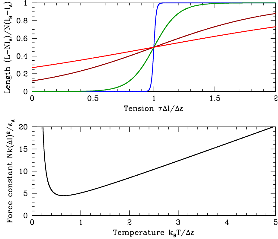
Figure 4.9: Upper panel: length L(\tau, T) for k_B T/\tilde{\varepsilon} = 0.01 (blue), 0.1 (green), 0.5 (dark red), and 1.0 (red). Bottom panel: dimensionless force constant k/N(\Delta\ell)^2 versus temperature.
