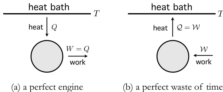
Figure 2.11: A perfect engine would extract heat Q from a thermal reservoir at some temperature T and convert it into useful mechanical work W . This process is alas impossible, according to the Second Law of thermodynamics. The inverse process, where work W is converted into heat Q , is always possible.
