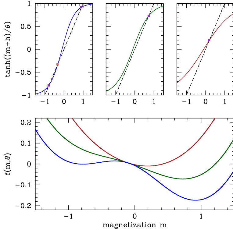
Figure 7.10: Results for h = 0.1 . Upper panels: graphical solution to the self-consistency equation m = \tanh((m+h)/\theta) at temperatures \theta = 0.65 (blue), \theta = 0.9 (dark green), and \theta = 1.5 (dark red). Lower panel: mean field free energy, with energy shifted by \theta \ln 2 so that f(m=0, \theta) = 0 .
