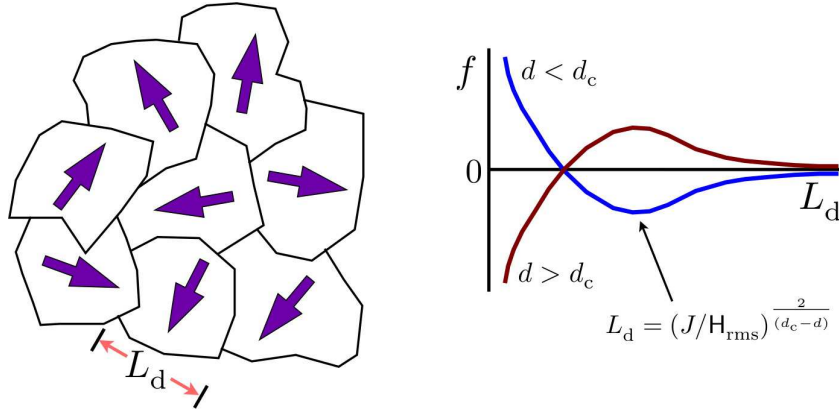
Figure 7.23: Left panel : Imry-Ma domains for an O(2) model. The arrows point in the direction of the local order parameter field \langle \hat{\mathbf{J}}(\mathbf{r}) \rangle . Right panel : free energy density as a function of domain size L_d . Keep in mind that the minimum possible value for L_d is the lattice spacing a .
