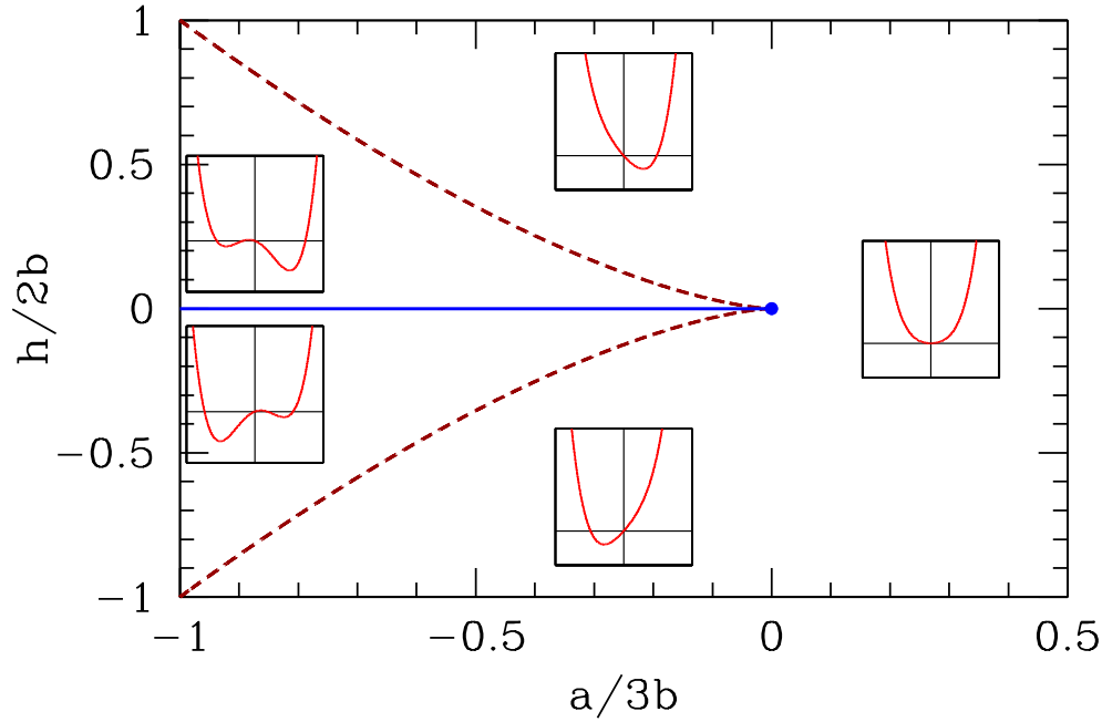
Figure 7.14: Phase diagram for the quartic Landau free energy f = f_0 + \frac{1}{2}am^2 + \frac{1}{4}bm^4 - hm , with b > 0 . There is a first order line at h = 0 extending from a = -\infty and terminating in a critical point at a = 0 . For |h| < h^*(a) (dashed red line) there are three solutions to the mean field equation, corresponding to one global minimum, one local minimum, and one local maximum. Insets show behavior of the free energy f(m) .
