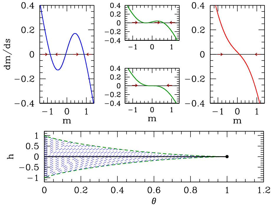
Figure 7.11: Dissipative magnetization dynamics \dot{m} = -f'(m) . Bottom panel shows h^*(\theta) from eqn. 7.67. For (\theta, h) within the blue shaded region, the free energy f(m) has a global minimum plus a local minimum and a local maximum. Otherwise f(m) has only a single global minimum. Top panels show an imperfect bifurcation in the magnetization dynamics at h = 0.0215 , for which \theta^* = 0.90 . Temperatures shown: \theta = 0.65 (blue), \theta = \theta^*(h) = 0.90 (green), and \theta = 1.2 . The rightmost stable fixed point corresponds to the global minimum of the free energy. The bottom of the middle two upper panels shows h = 0 , where both of the attractive fixed points and the repulsive fixed point coalesce into a single attractive fixed point (supercritical pitchfork bifurcation).
